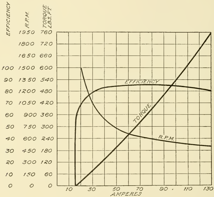
Fig. 45. Series Motor Characteristic Curves
